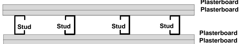
(b) Double layers of plasterboard lined steel frame wall panel
