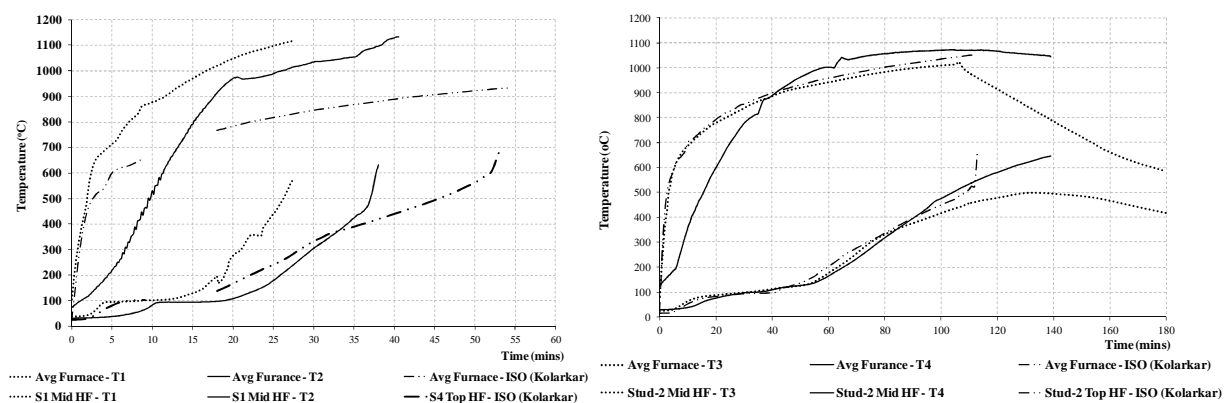
a. Specimens - T1, T2 and ISO834
